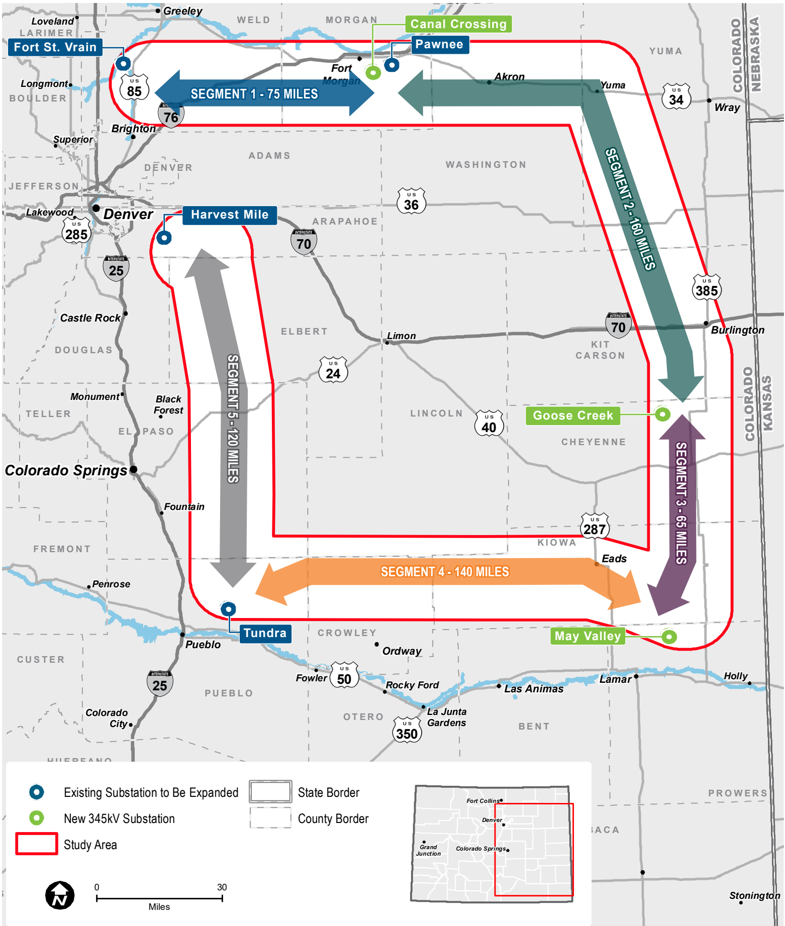
COLORADO'S POWER PATHWAY 345 KV TRANSMISSION PROJECT
